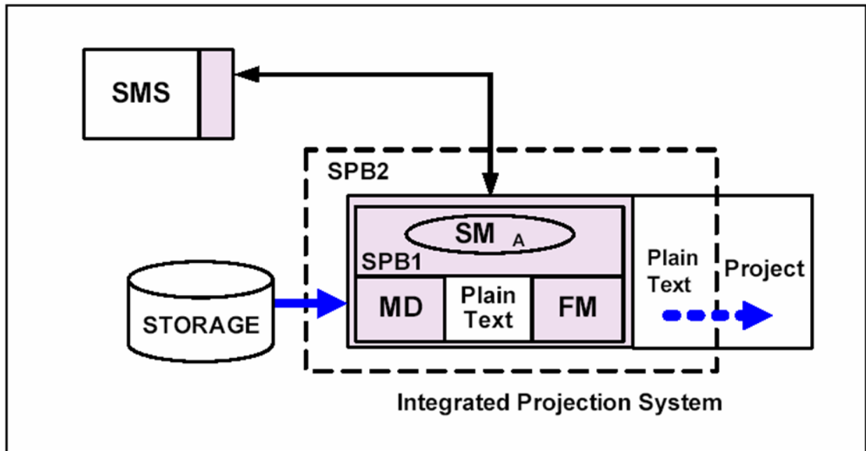
Figure 12: Media Block in Projector Configuration
